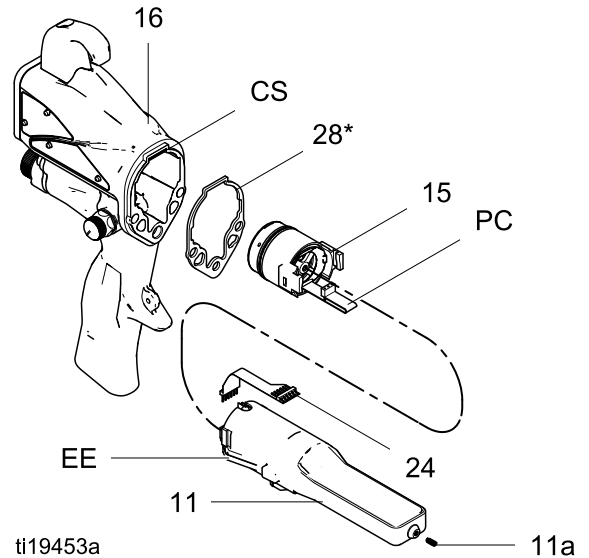
Figure 26 供电电源
