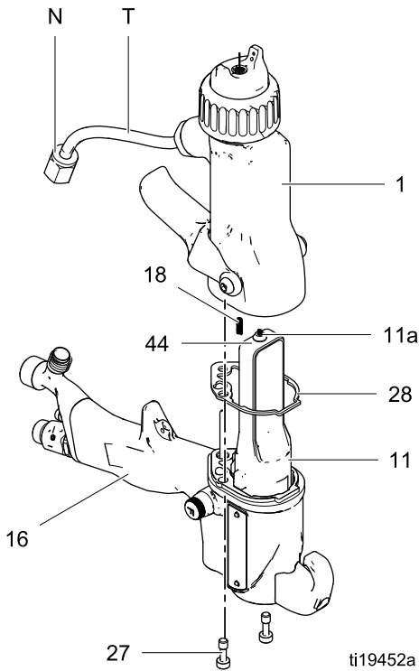
Figure 25 枪筒安装
