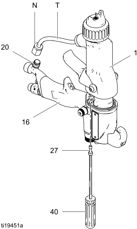
Figure 24 枪筒拆卸
