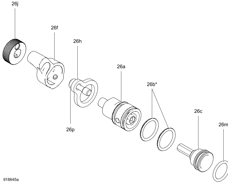
Figure 34 ES On-Off 和流体调节阀
