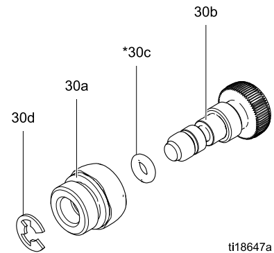
Figure 32 扇形空气调节阀
