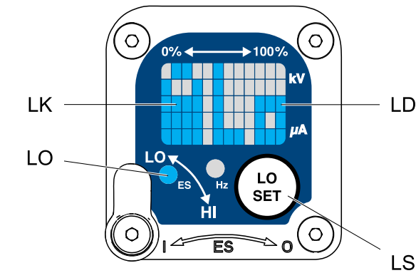
ti19339a Figure 9 低压锁定屏幕
