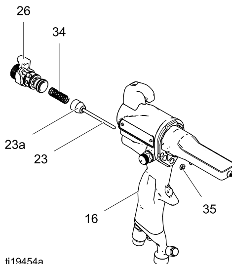
Figure 35 空气阀
