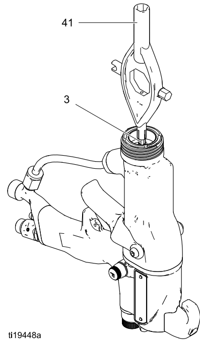
Figure 21 电极更换
