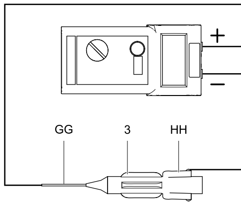
Figure 19 测试电极电阻
