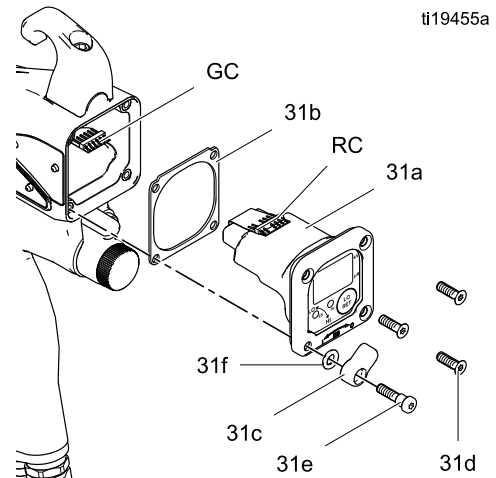
Figure 36 智能模块
