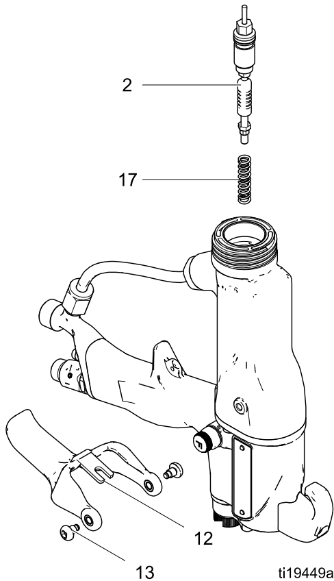
Figure 22 流体密封杆拆卸
