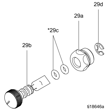
Figure 33 雾化空气限流阀
